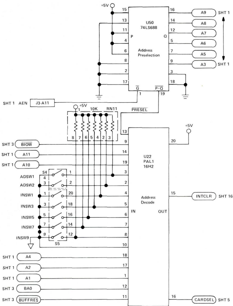
Address Decode
