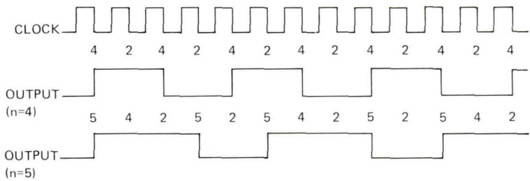
Mode 3: Square Wave Generator
