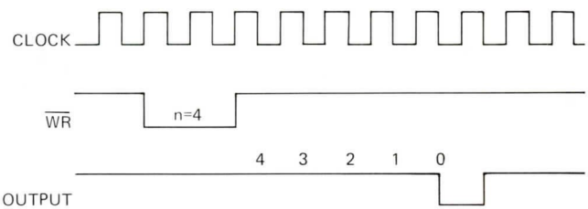
Mode 4: Software Triggered Strobe
